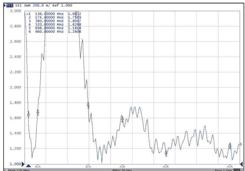
Measured by KEYSIGHT Network Analyzer E5063A
