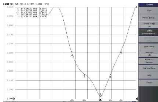
150-170 MHz VSWR vs. Freq.
