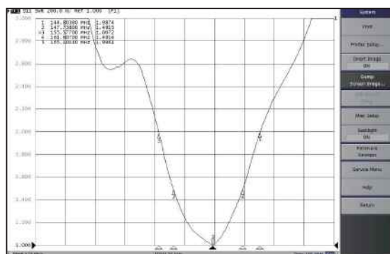
145-165 MHz VSWR vs. Freq.
